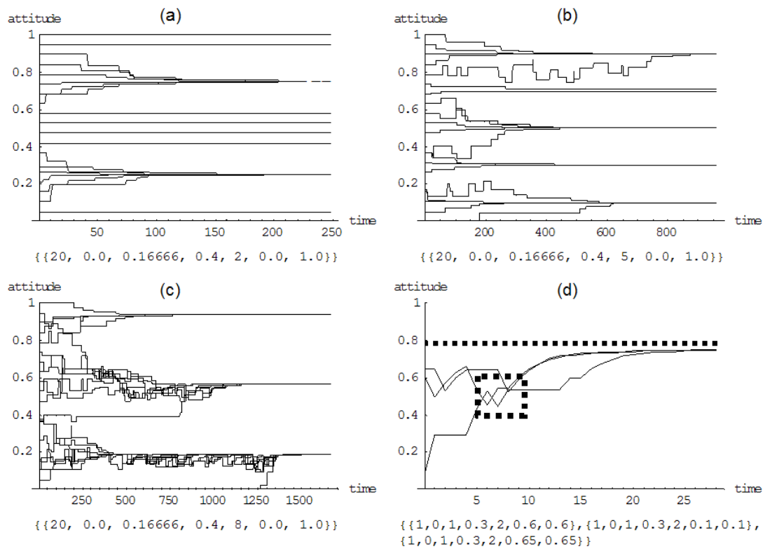
Figure 7: (a), (b), and (c) represent the three important scenarios for the analysis of the impact of precision: low, medium, and high precision. The setting of all three simulation runs is: 20 agents, no selective interpretation, a medium selective attention of 0.16666, and an impact rate of 0.4. Precision prec is 2 in (a), 5 in (b), and 8 in (c). Simulation run (d) exemplifies over adoption.
