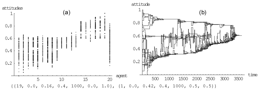
Figure 5: Dynamics with heterogeneous selective attentions: (a) shows all attitudes each of the 20 agents adopts during the simulation run, while (b) shows the sequential simulation run. Contrary to agents 1 to 19 that are narrow-minded with an equally small selective attention, agent 20 is open-minded, i.e. has a higher selective attention.
