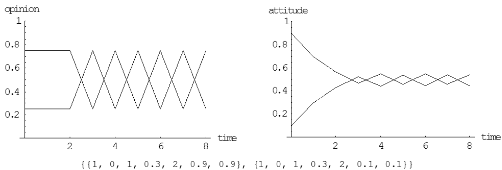
Figure 8: Cyclic over adoption: Simulation run with two agents, both without selective interpretation, both adopting every perceived opinion, both assigning an impact of 0.3 to perceived opinions, but each with another initial attitude.
